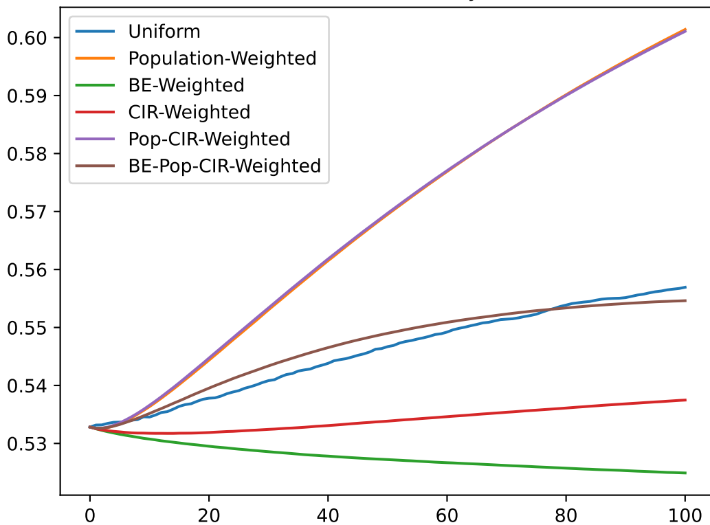
AZ, 2000: Red Player
